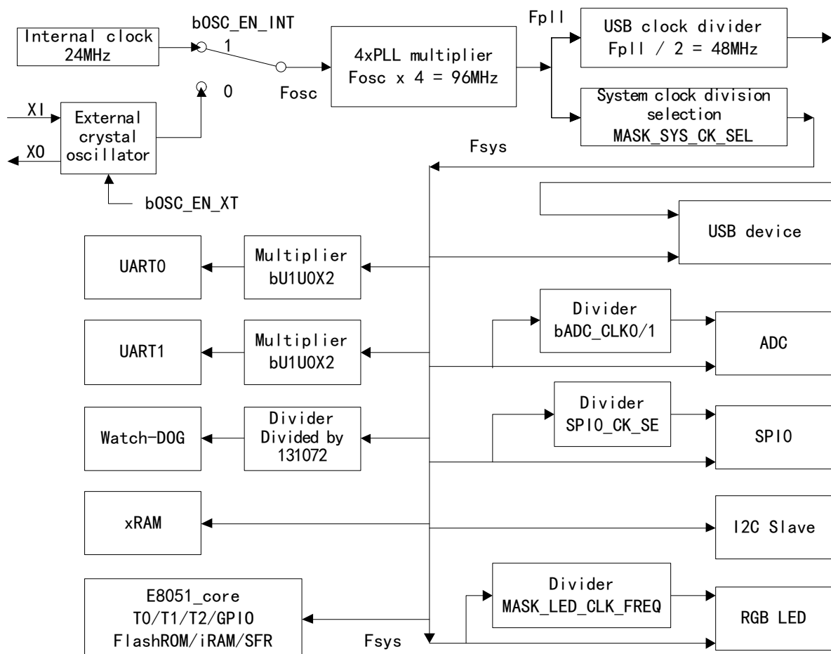
Figure 8.1.1 Clock System and Structure Chart
