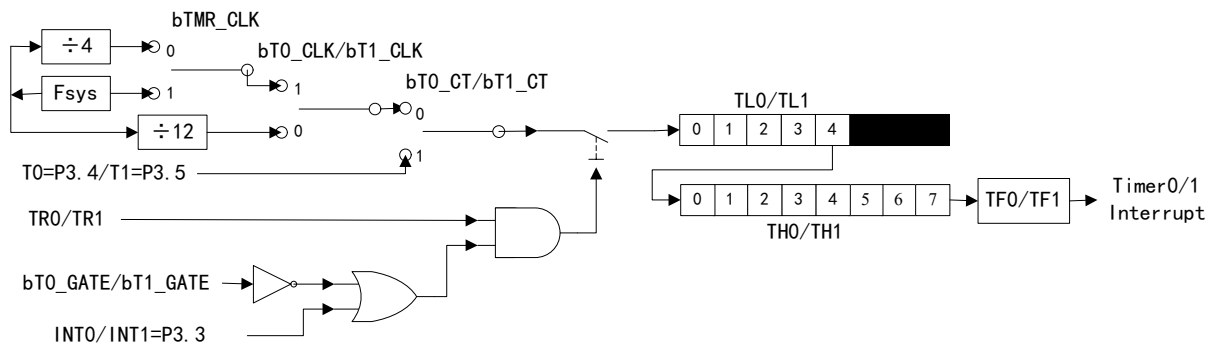
Figure 12.5.1.1 Timer0/1 mode 0
