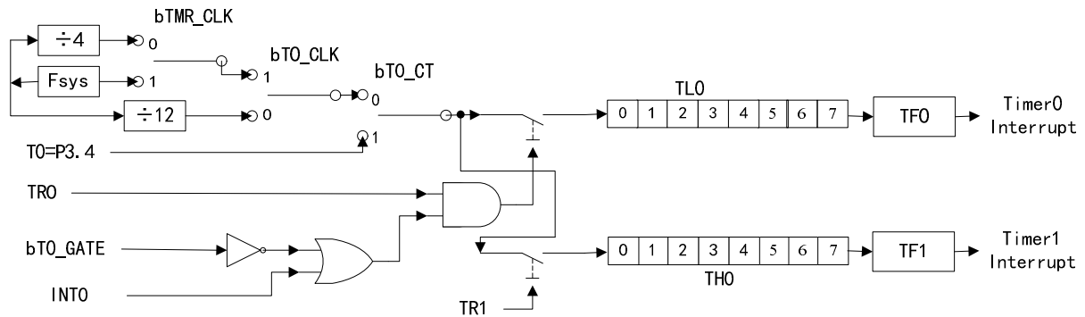
Figure 12.5.1.4 Timer0 mode 3
