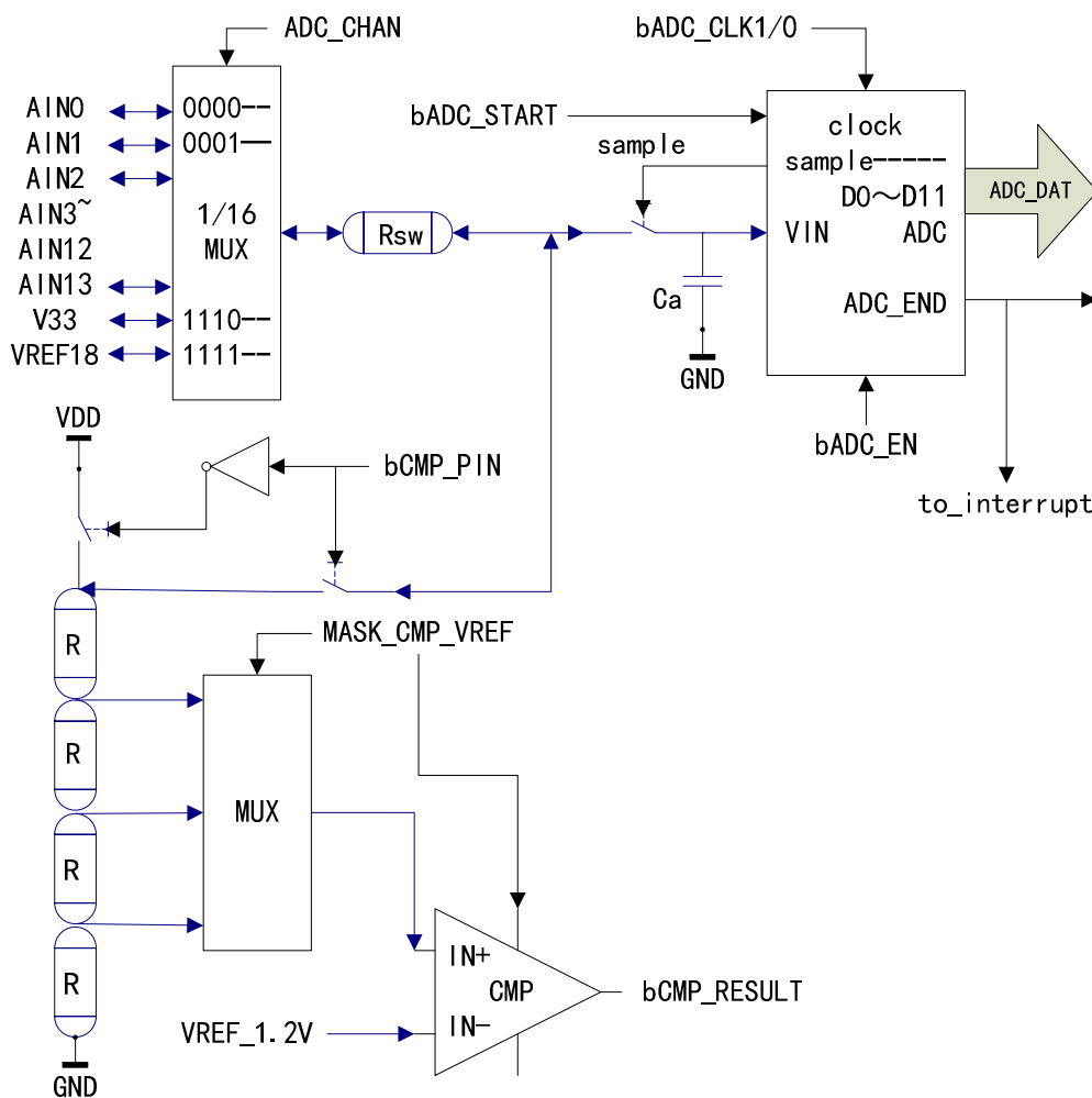
Figure 15.2.1 ADC structure diagram (Blue line represents analog signal)
