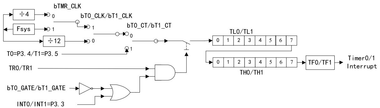
Figure 12.5.1.2 Timer0/1 mode 1
