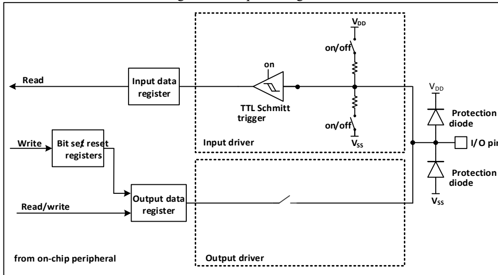
Figure 10-2 Input configuration
