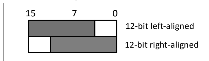
Figure 16-2 Data format
