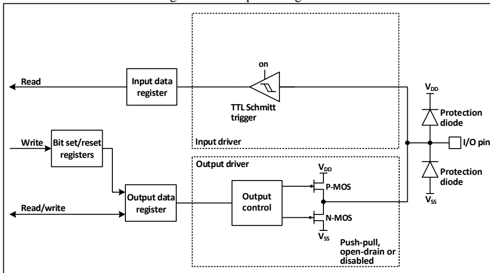
Figure 10-3 Output configuration
