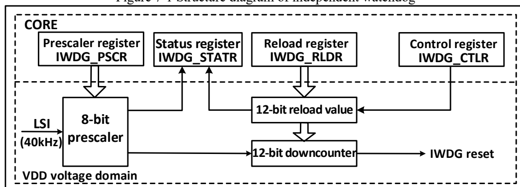
Figure 7-1 Structure diagram of independent watchdog
