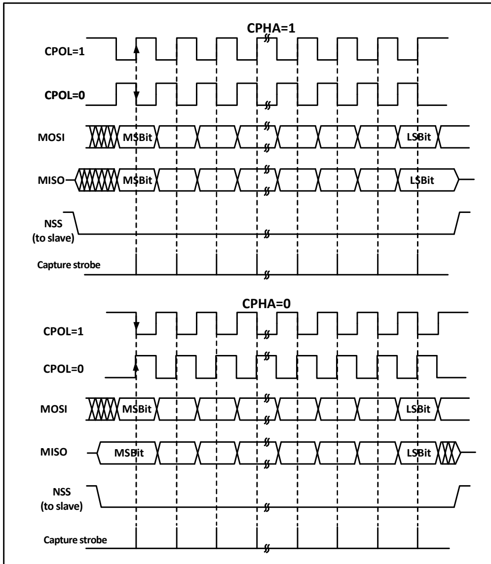
Figure 19-2 SPI mode
