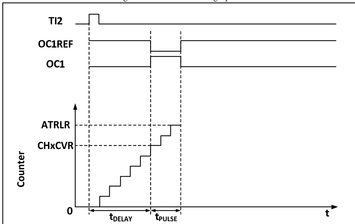
Figure 14-5 Generation of single pulse
