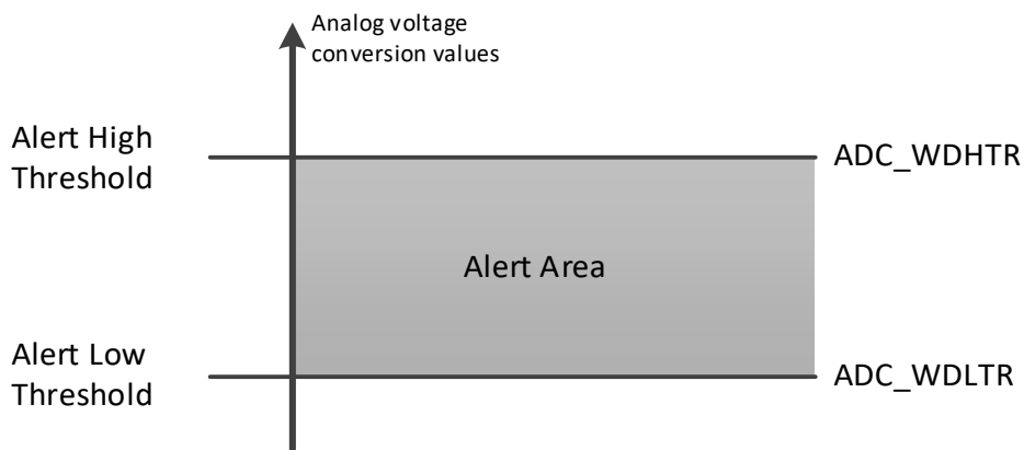
Figure 12-4 Analog watchdog guarded area
