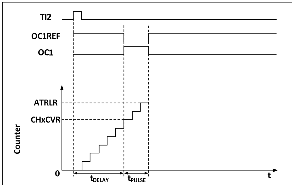
Figure 15-4 Event Generation and Pulse Response
