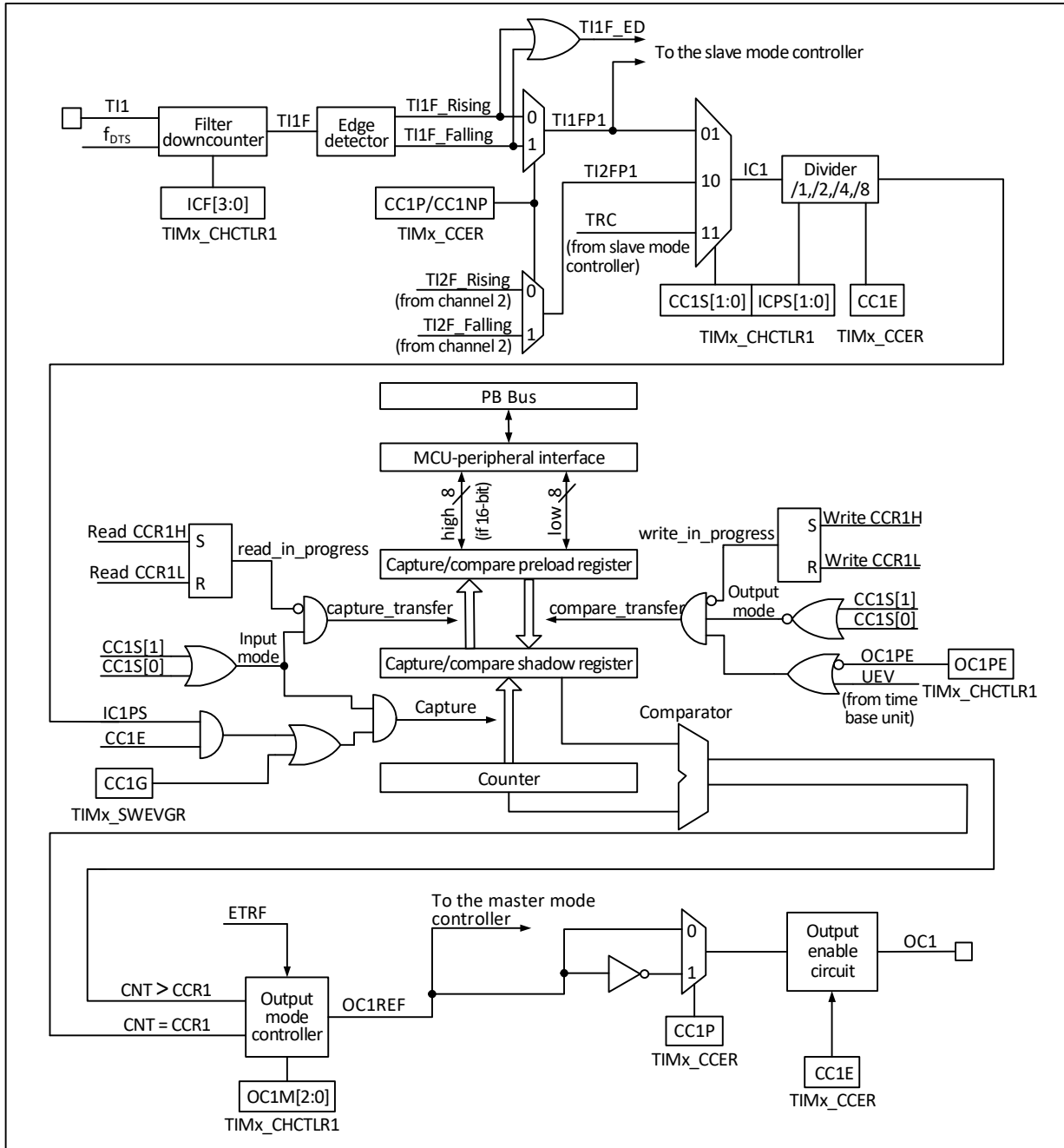
Figure 15-3 Structure block diagram of compare/capture
