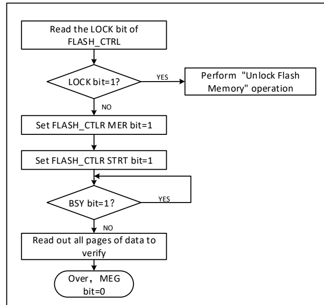
Figure 24-3 FLASH full chip erase
