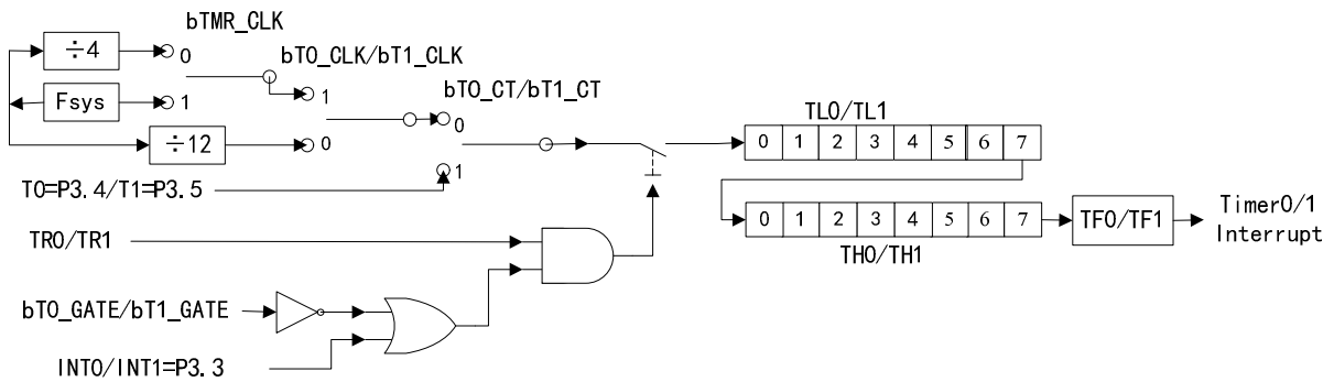
Figure 12.5.1.2 Timer0/1 mode1
