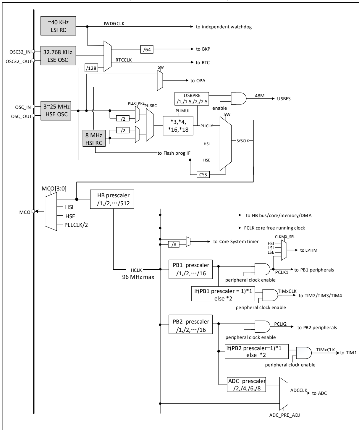
Figure 3-2 Clock tree block diagram
