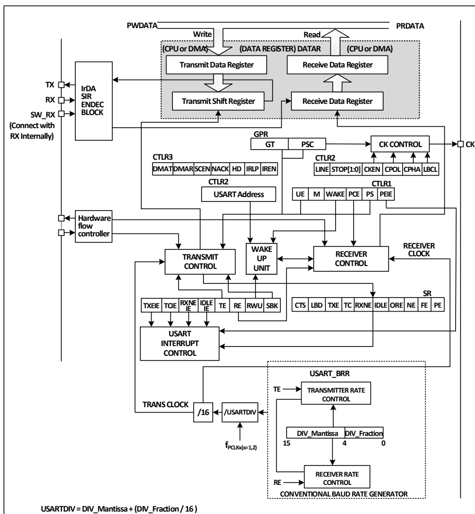
Figure 17-1 USART block diagram
