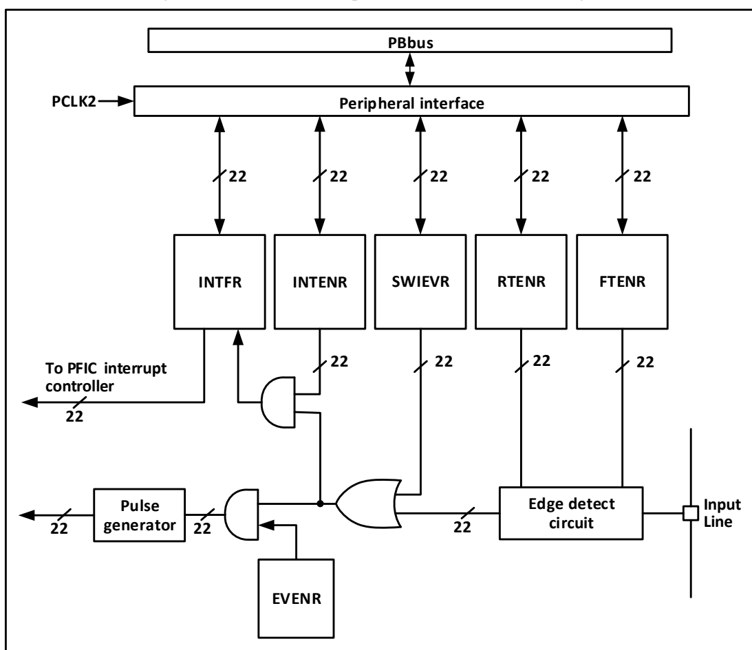
Figure 9-1 External interrupt (EXTI) interface block diagram
