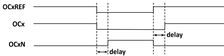
Figure 14-4 Complementary output and deadband
