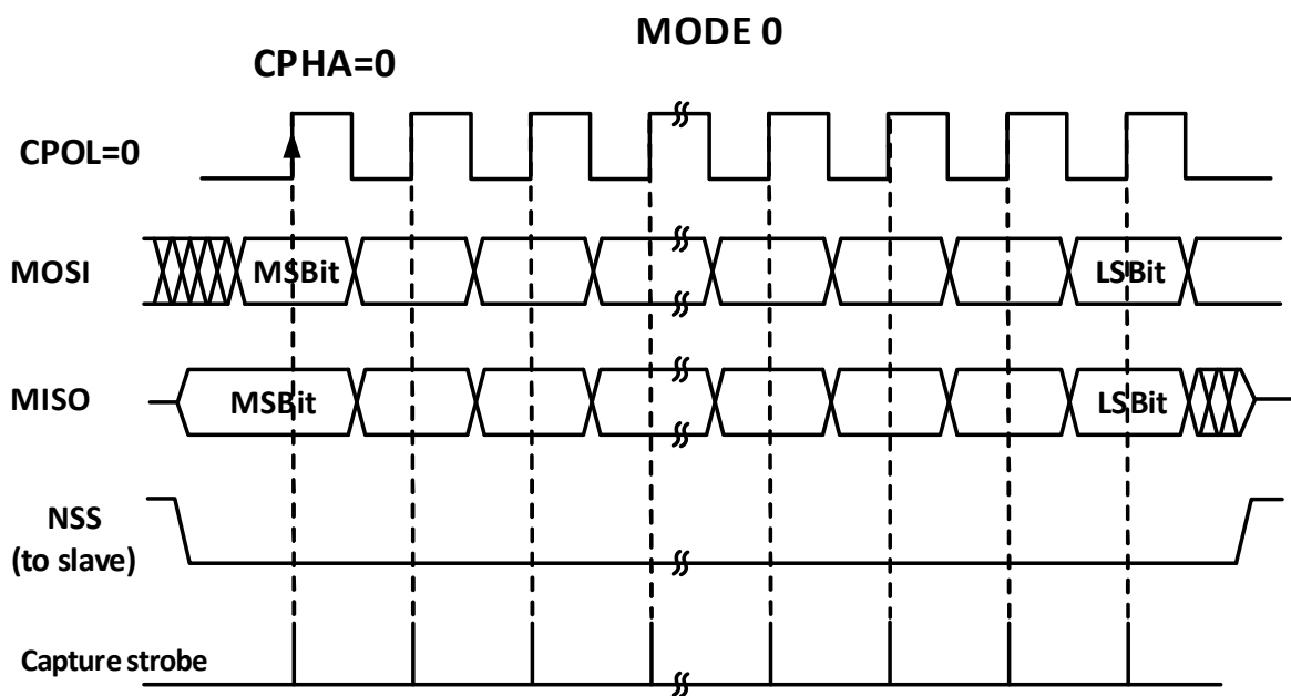
Figure 19-2 SPI master mode read/write mode 0
