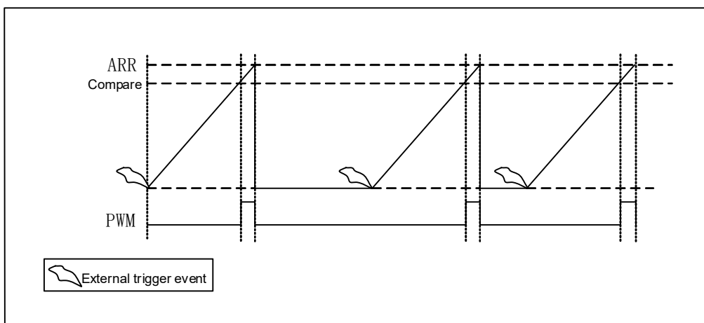
Figure 16-3 LPTIM output waveform, single count mode configuration
