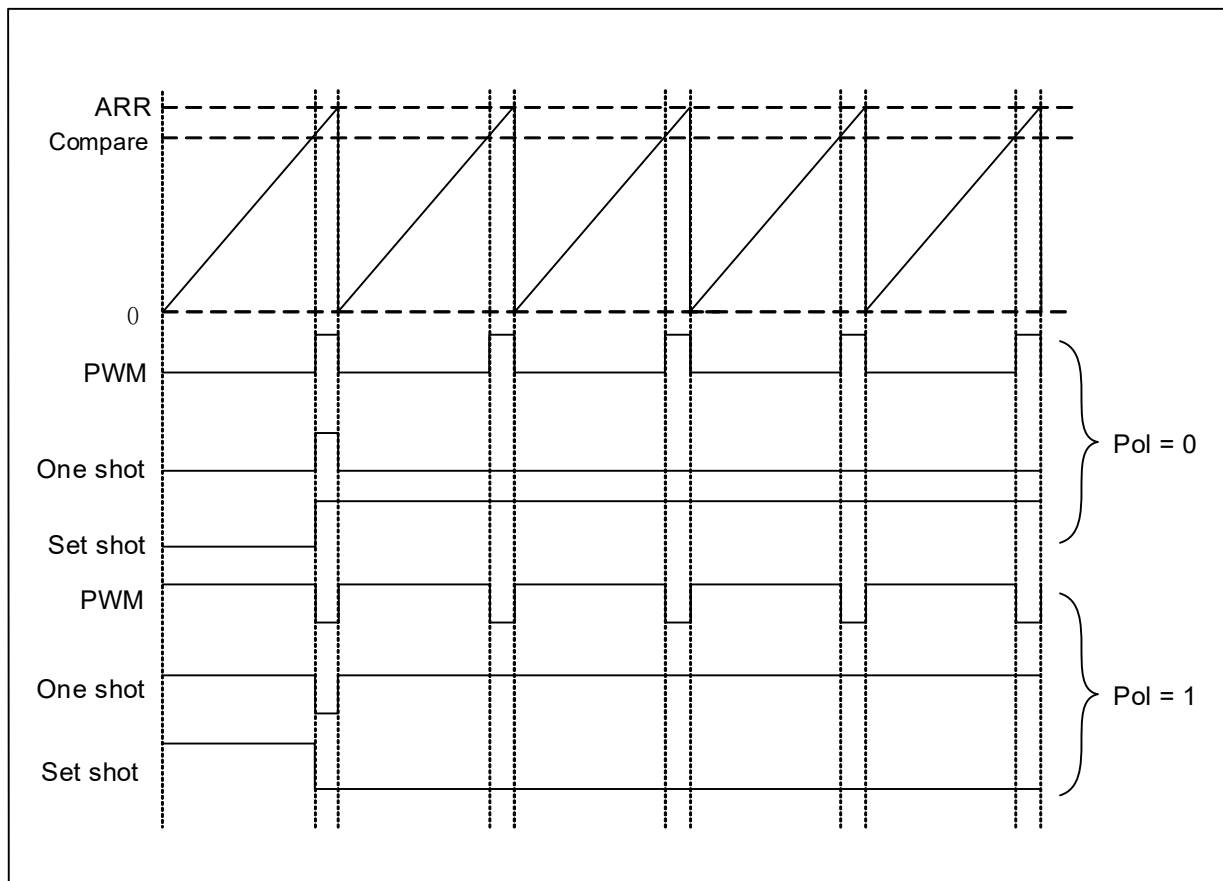
Figure 16-6 Waveform generation
