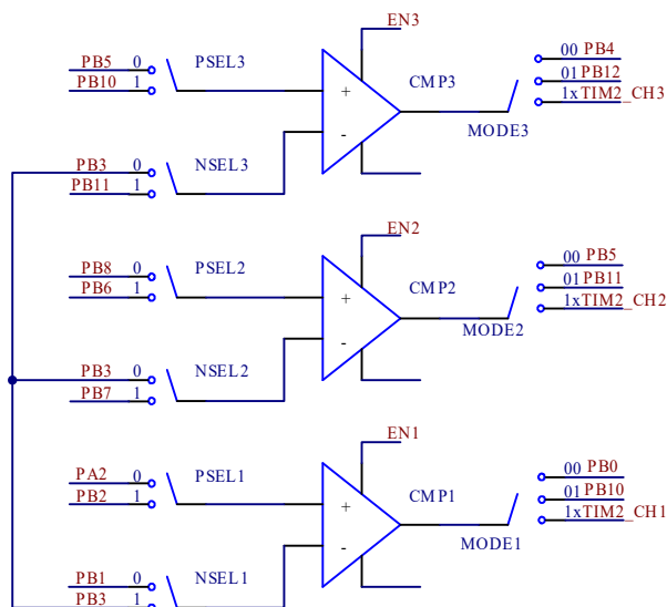
Figure 23-2 CMP Structure Diagram
