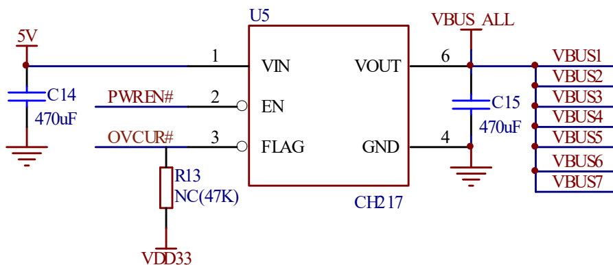
Figure 5-2 overall overcurrent detection and independent power control
