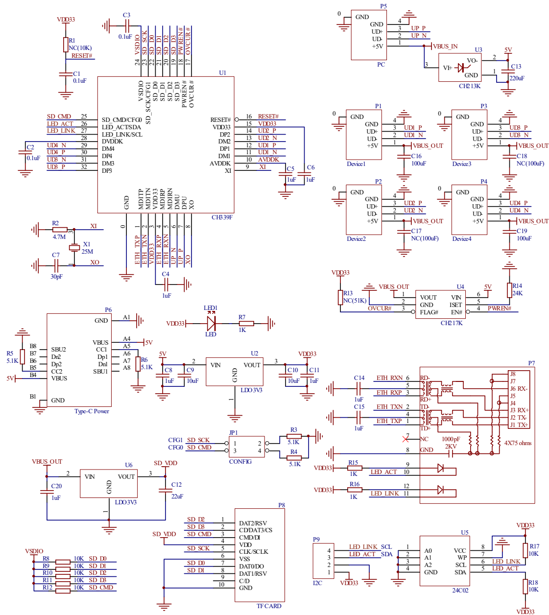
Figure 8-1 Reference circuit diagram for CH339F application
