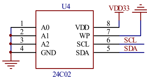
Figure 5-4 Schematic diagram of external EEPROM connection
