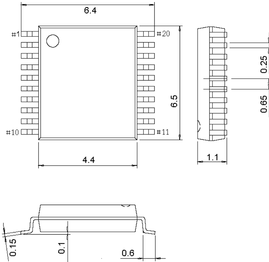
Figure 4-1 TSSOP20 package
