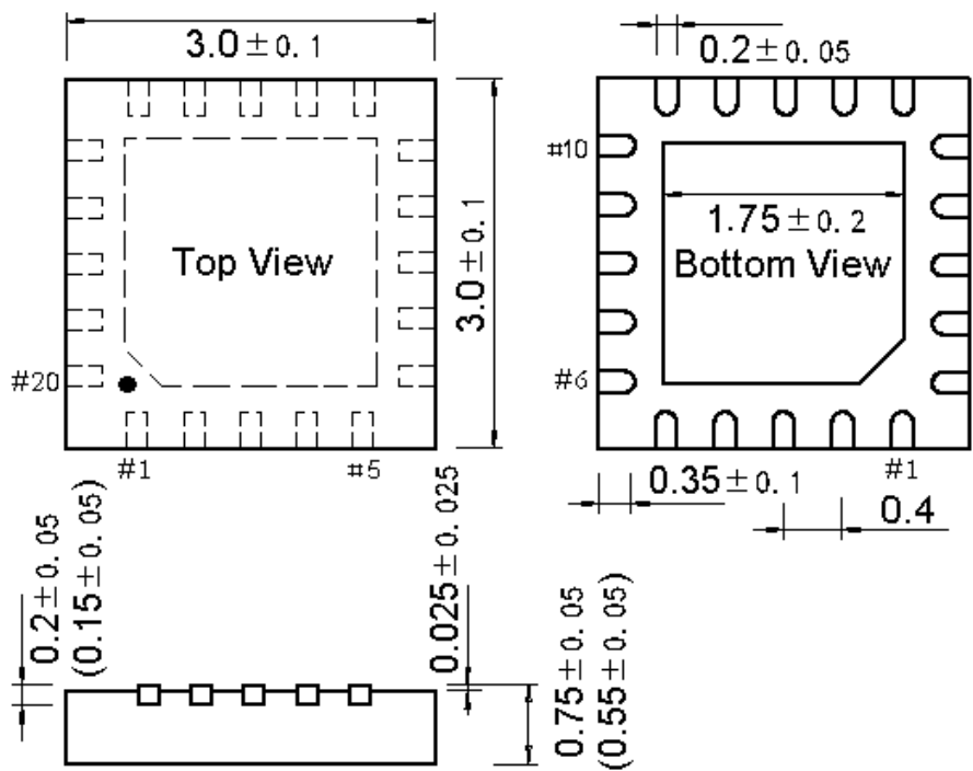
Figure 4-2 QFN20 package
