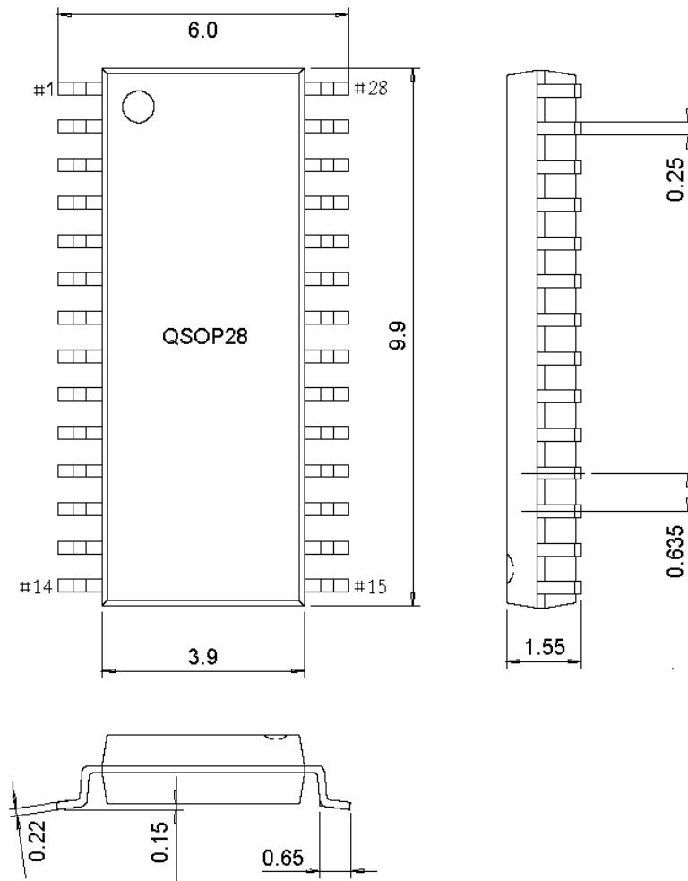
Figure 4-3 QSOP28 package
