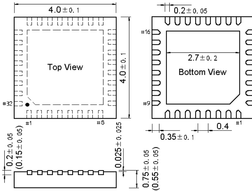
Figure 4-4 QFN32 package
