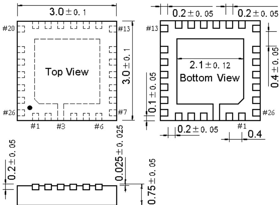
Figure 4-2 QFN26C3 package
