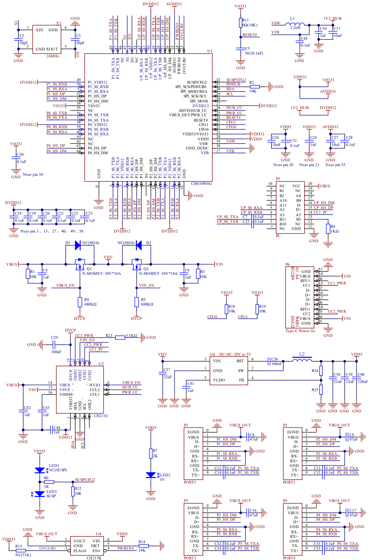
Figure 8-2 CH634W6G Chip reference circuit diagram
